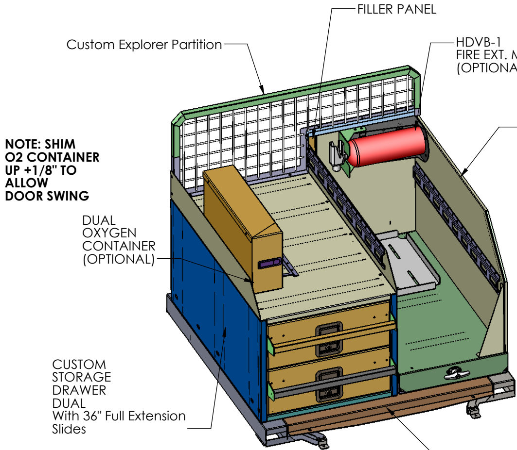
2013 FORD INTERCEPTOR UTILITY FULL SIZE CABINET SUB-FRAME (933-0099A)
