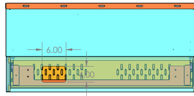
Cabinet Assy Rear View
