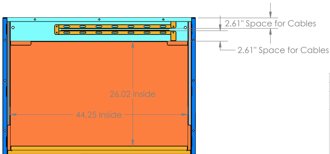
Bottom Dwr Closed Top View
