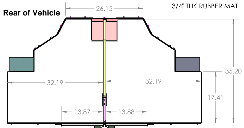
Downward View of the Floor Space SECTION B-B SCALE 1 : 16
